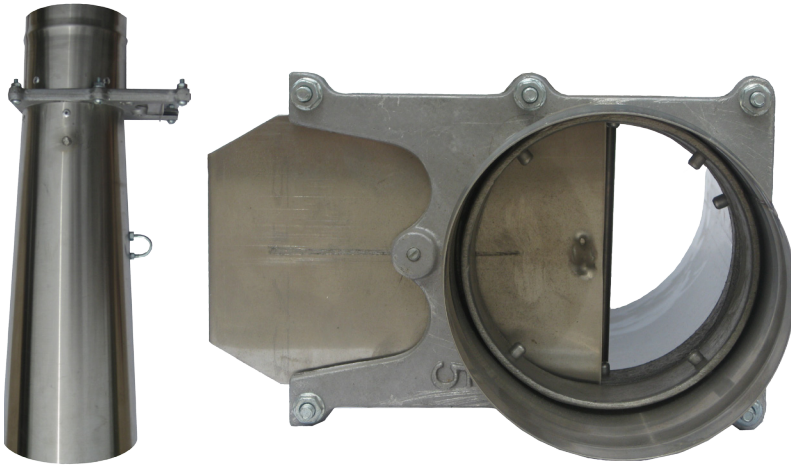
Diesel Stack - top view with air gate opened half way
